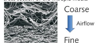
Hi Magnification photo showing the cross section of the Intrepid media
