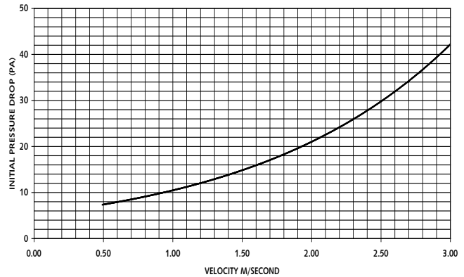
LINEAR VELOCITY M/SECOND VS PRESSURE DROP Metal Frame V Line Panel Filter 95mm Thick
