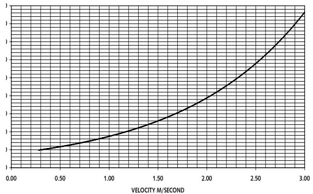
LINEAR VELOCITY M/SECOND VS PRESSURE DROP Metal Frame V Line Panel Filter 20mm Thick
