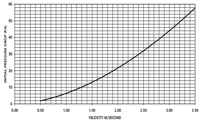
LINEAR VELOCITY M/SECOND VS PRESSURE DROP Metal Frame V Line Panel Filter 45mm Thick
