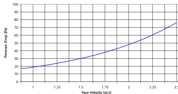
Pressure Drop vs/ Face Velocity Intrepid M82 Panel Filter 45mm Thick
