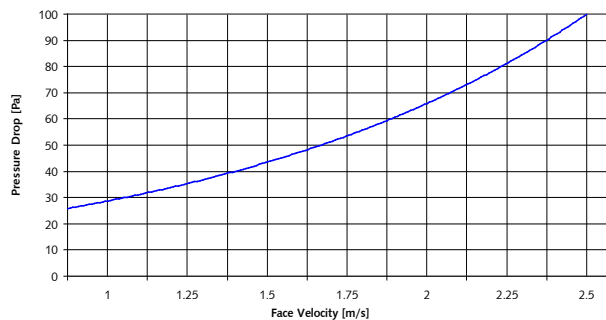
Pressure Drop vs/ Face Velocity Intrepid M81 Panel Filter 20mm Thick
