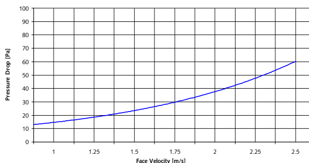
Pressure Drop vs/ Face Velocity Intrepid M84 Panel Filter 95mm Thick
